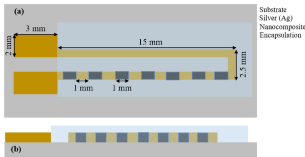
Fig. 1. Design of multi-stripes based deflection sensor, (a). Top View, (b) cross-sectional view.
