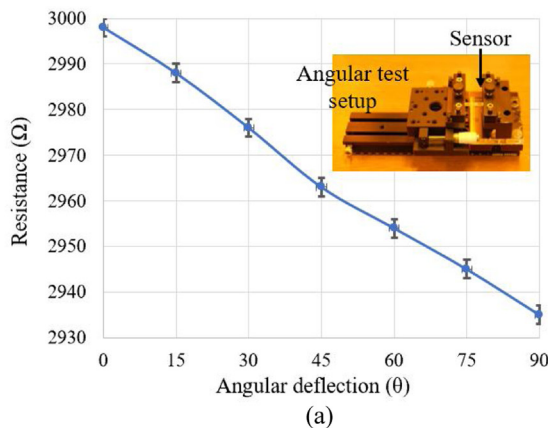
Fig. 7. (a) Sensor response in terms of resistance variation against various angular deflections and testing 20 times each at corresponding angle, (b) Sensitivity of the sensor.
